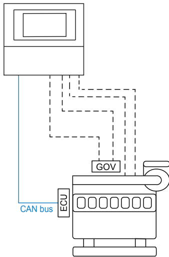
Engine drive
